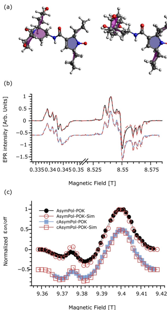
Figure 2. a) DFT-calculated structure of cAsymPol-OH viewed from the side, showing conformer #1 on the left and conformer #2 on the right. b) Concatenated X-band, 240 GHz EPR spectra and c) MAS-DNP field profile at 9.4 T for AsymPol-POK (black) and cAsymPol-POK (blue). The corresponding simulated EPR spectra and MAS-DNP field profiles are given as red dotted lines. For the MAS-DNP field profiles, experimental points are reported as circles for AsymPol-POK and squares for cAsymPol-POK, full for experiments and open for simulations.
