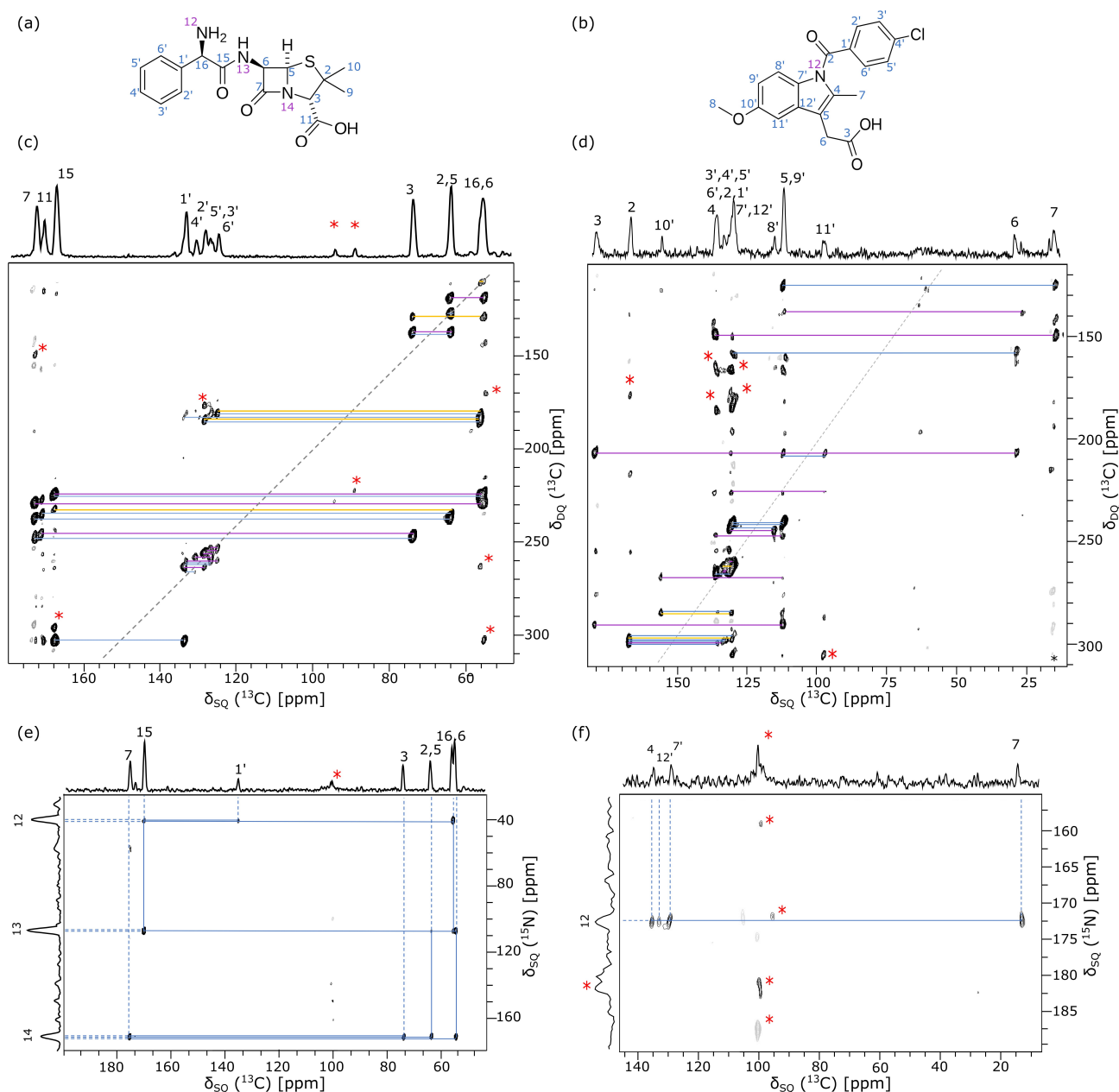
Figure 4. Molecular structures (a, b) and DNP-enhanced 2D ^{13}\text{C} - ^{13}\text{C} (c, d) and ^{15}\text{N} - ^{13}\text{C} (e, f) correlation spectra of ampicillin (a, c, e) and indomethacin (b, d, f) at NA. The DQ-SQ experiments in (c) and (d) were acquired using SR26 for dipolar recoupling, experiments in (e) and (f) were obtained with the zF-TEDOR sequence. All experiments were performed at 8 kHz MAS, 105 K and 9.4 T. Experimental times were 3 h for (b), 4 h for (c) and (d), and 5 h for (f). The ^{13}\text{C} assignment is mapped out in the 2D spectra, yielding one-bond (purple), two-bonds (blue) and three-bonds (yellow) correlations. Spinning side bands, signals from the carrier frequency and signals from the glycerol solvent are indicated with red asterisks.
