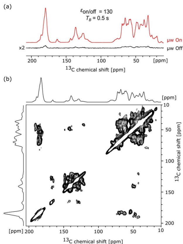
Figure 5. a) ^1\text{H} - ^{13}\text{C} CP-MAS spectra with (red) and without (black) \mu\text{w} irradiation of \text{U-}^{13}\text{C} , ^{15}\text{N} LecA, leading to an enhancement factor \epsilon_{\text{On/Off}} of 130. b) DNP-enhanced 2D SQ-SQ ^{13}\text{C} - ^{13}\text{C} correlation spectrum using the DARR sequence of the \text{U-}^{13}\text{C} , ^{15}\text{N} LecA. All spectra were acquired at a MAS frequency of 40 kHz, 9.4 T and 106 K.
