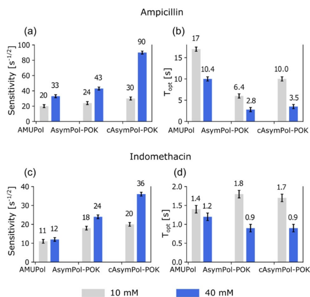
Figure 3. Experimental performance of a, b) ampicillin and c, d) indomethacin powders impregnated with 10 mM (grey) and 40 mM (blue) AMUPol, AsymPol-POK and cAsymPol-POK in the standard deuterated DNP matrix, d_8 -glycerol/ \text{D}_2\text{O} / \text{H}_2\text{O} (60:30:10 v/v), at 105 K, 9.4 T and 8 kHz MAS. The plots show the signal-to-noise ratio per square root of the experimental time ( S/N/\sqrt{t} ) in (a) and (c), and the optimal build-up time constant T_{\text{opt}} in (b) and (d) for ampicillin and indomethacin, respectively.
